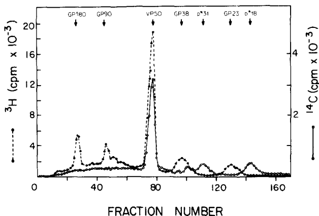
FIG. 3. Coelectrophoresis of the polypeptides of [ 3 H]valine (control, ●—●) and [ 14 C]valine (pronase treated, ○—○) labeled coronavirus A59 virions. Virus was grown for 34 hr in the presence of 4 \mu Ci/ml of [ 3 H]valine or 1 \mu Ci/ml of [ 14 C]valine. Purified [ 14 C]valine-labeled virus was treated with pronase, 2 mg/ml, for 2 hr at 37° and repurified (see Materials and Methods for details). Pelleted pronase-treated virions resuspended in complete Laemmli buffer were heated to 100° for 2 min and mixed with [ 3 H]valine-labeled control virus which had been boiled for 2 min.
