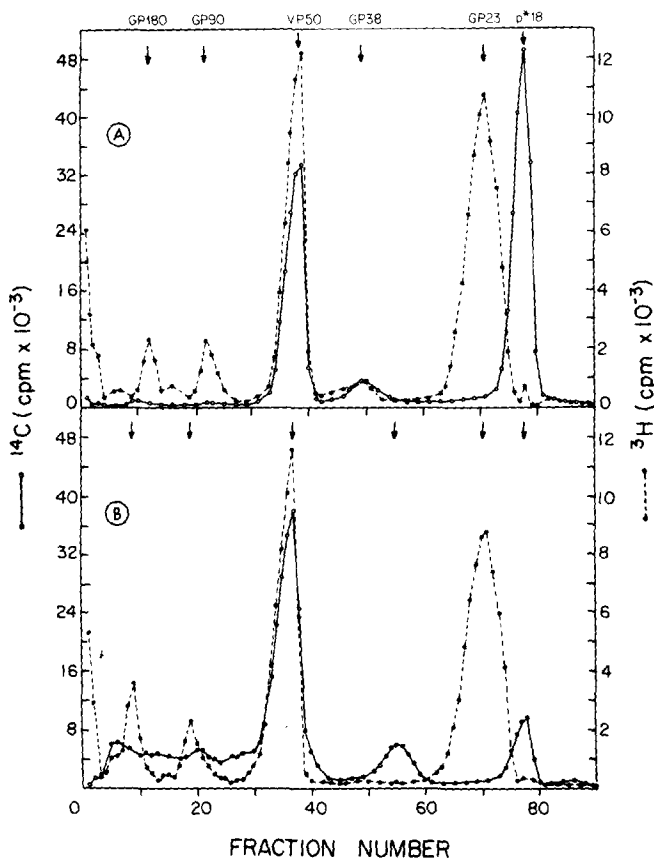
FIG. 7. Effects of boiling and \beta -MSH on the electrophoretic pattern of bromelain-treated A59 virion polypeptides; coelectrophoresis of the polypeptides of [^3\text{H}] valine-labeled (control, \bullet — \bullet ) and [^{14}\text{C}] valine-labeled (bromelain-treated, \circ — \circ ) virions. A59 virus was grown for 24 hr in the presence of 4\ \mu\text{Ci/ml} of [^3\text{H}] valine or 1\ \mu\text{Ci/ml} of [^{14}\text{C}] valine. Purified [^{14}\text{C}] valine-labeled virions were incubated at 37^\circ for 3 hr in TMEN (pH 6) with 1\ \text{mg/ml} of bromelain plus 0.1\ \text{mM} \beta -MSH; [^3\text{H}] valine-labeled virus was kept at 4^\circ in TMEN (pH 6). Both preparations were repurified (see Materials and Methods) and treated as follows: to one half of the bromelain-treated [^{14}\text{C}] -labeled virus, SDS, glycerol, and BPB were added to final concentrations of 2%, 10%, and 0.001%, respectively. This sample was mixed with one half of the [^3\text{H}] valine-labeled untreated virus similarly diluted at room temperature, and the mixture was placed immediately on a gel. The remainder of the bromelain-treated [^{14}\text{C}] valine-labeled virus received 2% SDS, 10% glycerol, 0.001% BPB, and 5% \beta -MSH and was boiled for 5 min. After cooling to room temperature, the sample was mixed with the remainder of the [^3\text{H}] valine-labeled untreated virus which was resuspended in SDS with glycerol and BPB at 25^\circ , and these were coelectrophoresed on a second gel. (A) bromelain-treated and untreated virus, both samples unheated, no \beta -MSH; (B) bromelain-treated virus heated at 100^\circ for 5 min with 5% \beta -MSH; untreated virus, unheated, no added \beta -MSH before mixing with the bromelain-treated sample.
