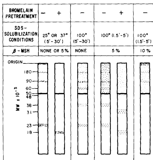
GEL PATTERN AND APPARENT MOLECULAR WEIGHTS OF POLYPEPTIDES
