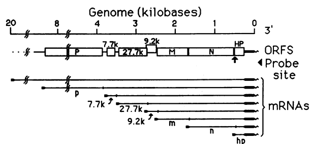
FIG. 1. Structural relationships among the genome, mRNA transcripts, and synthetic oligodeoxynucleotide probes. The seven open reading frames (ORFs) deduced from primary sequence of the 3' end of the TGEV genome are drawn to scale. They are identified as P for peplomer protein, M for matrix protein, N for nucleocapsid protein, HP for hydrophobic protein, and 7.7k, 27.7k, and 9.2k for potential nonstructural proteins of 7.7, 27.7, and 9.2 kDa, respectively. Their corresponding mRNAs are identified as p, m, n, hp, 7.7k, 27.7k, and 9.2k. The site from which the oligonucleotide probes were derived is indicated by an arrow. The 5' leader sequence (presumed to be 80 bases) and the 3' noncoding sequence (276 bases) are indicated by heavy lines and are drawn to scale. The 3' poly(A) tail is indicated by a wavy line. The largest mRNA, which serves as template for synthesis of the viral polymerase, is presumably identical to the genome.
