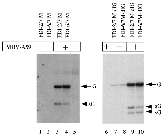
FIG. 6. Northern blot analysis of insertion mutants. Intracellular RNAs were extracted from DI RNA-transfected, MHV-infected cells (lanes 3, 4, 9, 10) or DI RNA-transfected, mock-infected cells (lanes 1, 2, 7, 8). Lanes 5 and 6 represent RNA from MHV-infected cells. Poly(A)-containing RNAs were analyzed by Northern blot analysis using probe 2 (see Fig. 5). Arrowhead and arrow point to subgenomic DI RNAs and genomic DI RNAs, respectively. The minute amount of genomic DI RNA-sized signal in lanes 7 and 8 represents the transfected DI RNA transcripts that were not degraded in MHV-uninfected cells.
