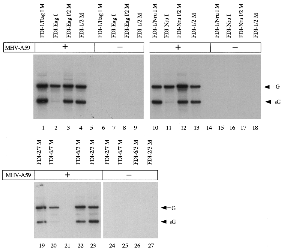
FIG. 4. Northern blot analysis of insertion mutants. Intracellular RNAs were extracted from DI RNA-transfected, MHV-infected cells (lanes 1–4, 10–13, 19, 20, 22, 23) or DI RNA-transfected, mock-infected cells (lanes 6–9, 15–18, 24–27). Lanes 5, 14, and 21 represent RNA from MHV-infected cells. Poly(A)-containing RNAs were analyzed by Northern blot analysis using probe 1 (see Fig. 1). Arrowhead and arrow point to subgenomic DI RNAs and genomic DI RNAs, respectively.
