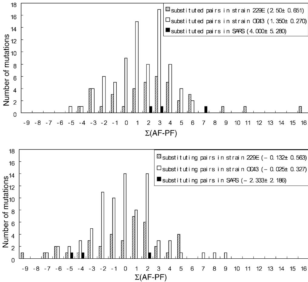
Fig. 2. Sum of differences between actual and predicted frequencies in substituted and substituting amino acid pairs in the spike proteins from different human coronaviruses (the data are presented as mean \pm S.E.).
