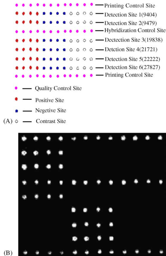
Fig. 3. SARS universal microarray. (A) Spotting design of the universal microarray. The color is added artificially in order to distinguish the different sites. (B) Detection results of a sample.
