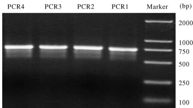
Fig. 2. The electrophoresis graph of the PCR products. The PCR products in the picture: PCR1, PCR2, PCR3 and PCR4 is relative to the numbers (Table 3): 1, 2, 3 and 4, respectively.
