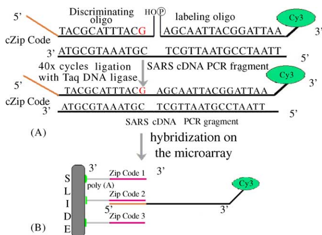
Fig. 1. The schematic of the universal microarray-mediated by LDR. (A) The genotype of every mutation base can be detected by a set of oligonucleotides including a discriminating oligonucleotide and a labeled oligonucleotide. The discriminating oligonucleotide contains a cZip Code at 5' end and a hydroxy group at 3' end. The labeled oligonucleotide was phosphorylated at 5' end and is affixed a Cy3 to 3' end. The two sequences at the junction must be matched. (B) The spotting sequences consist of a Zip Code at the 5' end and the (dA) 15 -NH 2 H 21 at 3' end; the discriminating oligonucleotide includes cZip Code at the 5' end and the hybridization sequence at 3' end.
