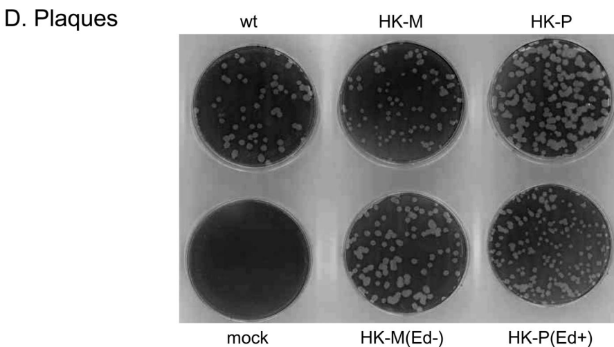
FIG. 3. MHV S protein endodomain mediates the incorporation of Hook protein into MHV virions. (A) Amino acid composition of the carboxy termini of four Hook protein constructs. The four types of mutants were HK-M, containing the transmembrane domain and endodomain from the MHV S protein; HK-M(E d -), identical to HK-M with a truncated endodomain; HK-P, containing the transmembrane domain and endodomain from PDGFR (as in the original Hook construct [Fig. 1]); and HK-P(E d +) , identical to HK-P but with the PDGFR endodomain replaced with the endodomain of the MHV S protein. Transmembrane domain residues are shown in bold; underlined residues are part of the adjacent Myc epitope tag in the ectodomain. (B and C) Western blots of lysates from cells infected with Hook protein mutants (B) or of purified virions of Hook protein mutants (C). The Hook protein was detected with an antibody for the HA epitope tag; the amounts of lysate or virion samples analyzed were normalized to contain equivalent amounts of N protein, as detected by an anti-N antibody. (D) Plaques formed by viruses encoding the four variant Hook proteins. Wild-type MHV and the mutants HK-M, HK-M(E d -), HK-P, and HK-P(E d +) were titrated on mouse L2 cell monolayers, stained with neutral red at 44 h postinfection, and photographed 8 h later.
