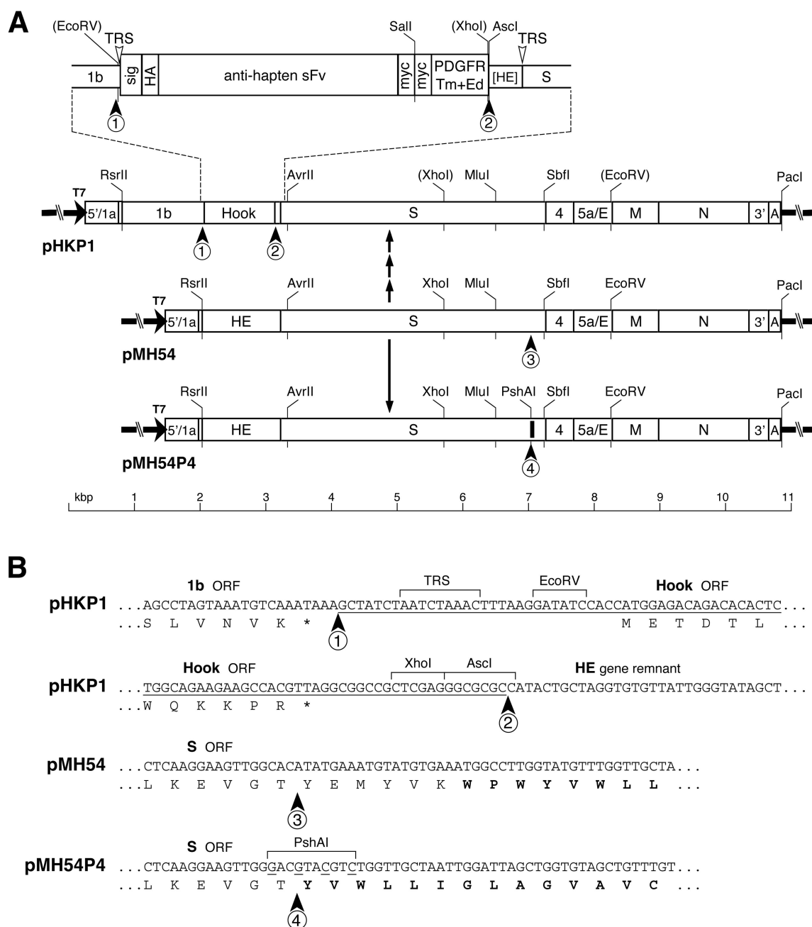
FIG. 1. Transcription vectors for synthesis of donor RNAs used in the construction of transmembrane domain and endodomain mutants. (A) Plasmids pHKP1 and pMH54P4 were derived from pMH54 (24), as detailed in Materials and Methods. In each plasmid schematic the arrow denotes the T7 promoter, and the restriction sites shown are those relevant to plasmid construction; all restriction sites, except for those in parentheses, are unique in the plasmid in which they appear. The solid rectangle in pMH54P4 indicates the 27-nt deletion. The expanded section of pHKP1 shows the elements encoded by the Hook gene: the signal peptide (sig), the influenza virus HA epitope tag, the anti-hapten single-chain antibody (sFv) fragment, two copies of the Myc epitope tag, and the transmembrane domain (Tm) and endodomain (Ed) from PDGFR. Also indicated are the TRSs preceding the Hook and S genes. HE, 99-nt remnant of the HE gene. Mutated derivatives of each parent plasmid were constructed by the insertion of PCR-generated fragments into the Sall-Ascl and PshAI-SbfI intervals of pHKP1 and pMH54P4, respectively. (B) DNA sequences of the four junctions that are labeled in panel A. 1 and 2, the upstream and downstream boundaries of the Hook gene insertion in pHKP1, including the introduced TRS for the Hook open reading frame and relevant restriction sites; 4, the PshAI site and 27-nt deletion created in pMH54P4 between the S gene ectodomain and transmembrane domain; 3, the wild-type counterpart of junction 4 in pMH54. Underlined nucleotides are non-MHV sequences, including base changes created to introduce restriction sites. Shown beneath the DNA sequences are translations of portions of the 1b, Hook, and S open reading frames (with asterisks denoting stop codons); for pMH54 and pMH54P4, amino acid residues in bold are in the transmembrane domain of the S protein.
