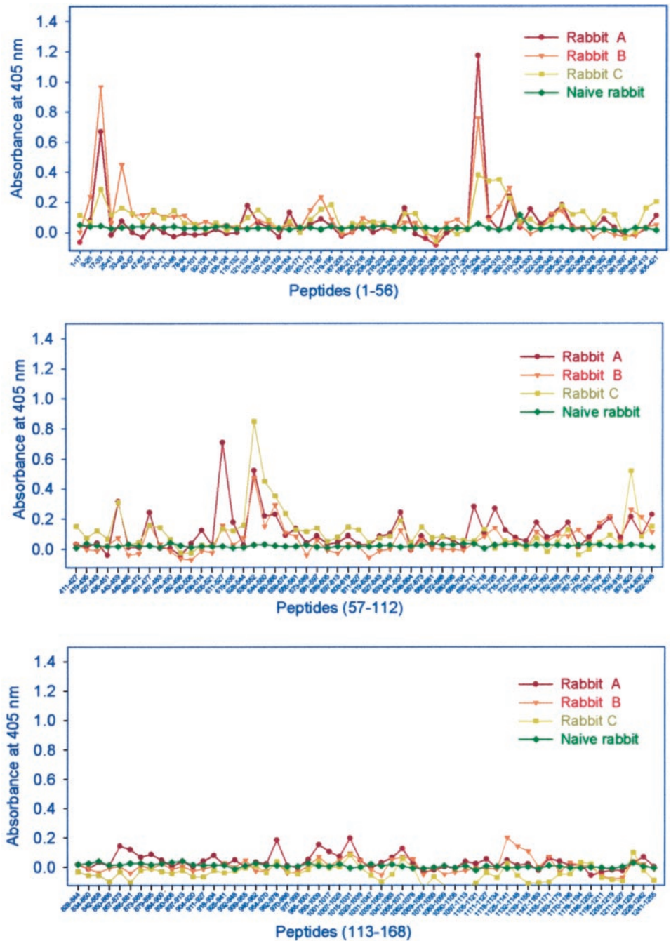
FIGURE 5. Pepsican analysis against the antisera from rabbits immunized with inactivated SARS-CoV. Reactivity of the rabbit antisera at 1/100 dilution with the peptides overlapping the entire sequences of the S protein was measured by ELISA.
