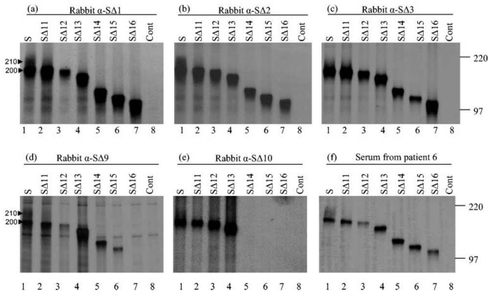
FIG. 3. Radiolabeled immunoprecipitation. Cos7 cells were transfected with plasmids expressing full-length S and the C-terminally truncated S proteins, S \Delta 11, S \Delta 12, S \Delta 13, S \Delta 14, S \Delta 15, and S \Delta 16 (lanes 1, 2, 3, 4, 5, 6, and 7) or with a plasmid without an insert as a negative control (lanes 8). ^{35} S-labeled S proteins were immunoprecipitated with the antibodies indicated (top of each autoradiograph) and then separated in SDS-7.5% PAGE gels. Arrowheads (left), molecular masses (in kilodaltons) of specific S proteins. High-range Rainbow molecular weight markers (right; Amersham) were used. \alpha , anti.
