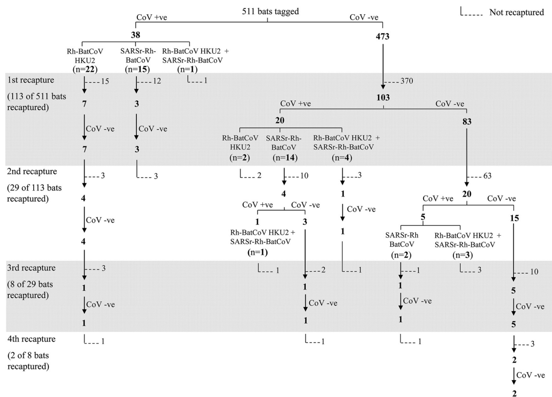
FIG. 2. Schematic diagram showing the number of Rhinolophus sinicus (Chinese horseshoe) bats tagged and recaptured, and the presence of coronaviruses among these tagged bats. The numbers in bold type indicate the number of bats successfully recaptured. The numbers in roman type (not boldface type) following dashed lines are the numbers of bats not recaptured in subsequent visits. The numbers in parentheses are the number of recaptured bats positive for coronaviruses. CoV +ve, coronavirus positive; CoV -ve, coronavirus negative.
