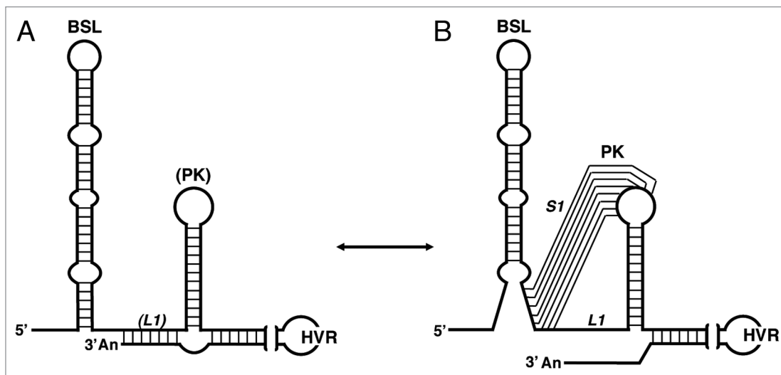
Figure 3. Alternative RNA structures at the MHV 3' UTR. Two RNA motifs that probably exist in a dynamic equilibrium are shown. The switch between both structures has been postulated in the initiation of CoV RNA synthesis. 75 (A) 3' UTR structure in which the BSL is folded and the 3' end is annealed to the base of PK loop ( L1 ). (B) 3' UTR conformation in which the 3' end is released and the lower stem of BSL is disrupted leading to the formation of the PK. BSL, bulged stem-loop; PK, pseudoknot; S1 and L1 , stem 1 and loop 1 of the pseudoknot; HVR, hypervariable region. Acronyms as in Figure 2.
