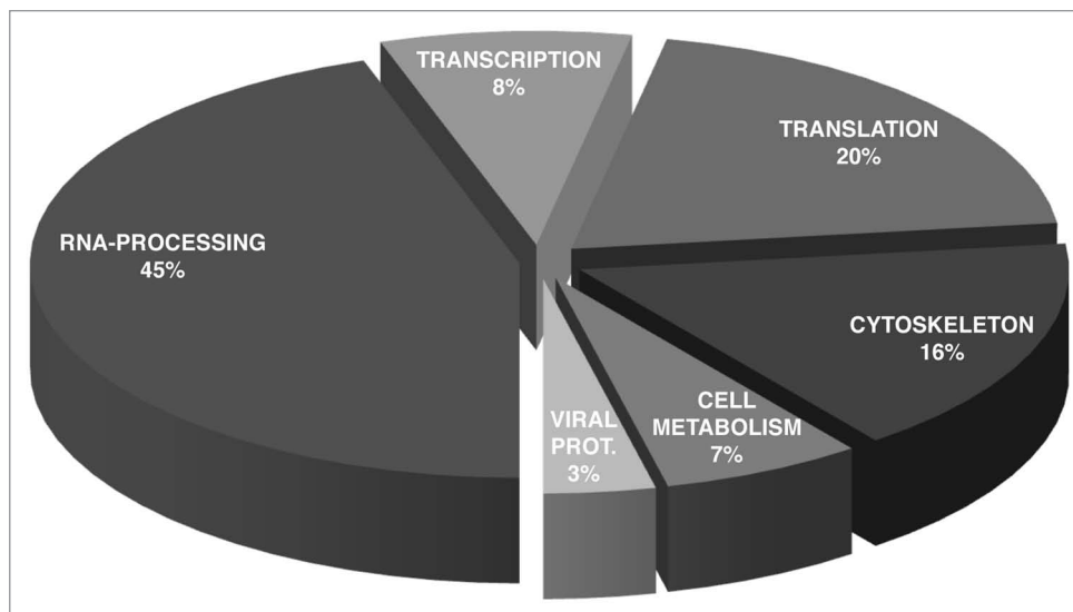
Figure 6. Cell proteins with affinity for TGEV RNA structural motifs. Functional classification of cellular proteins interacting with CoV TRSs. RNA-affinity chromatography assays were performed with TGEV-infected human Huh7 cell extracts and viral TRS RNAs. Forty proteins interacting with TRS RNAs were identified by mass spectrometry and categorized according to the biological processes in which they are involved.
