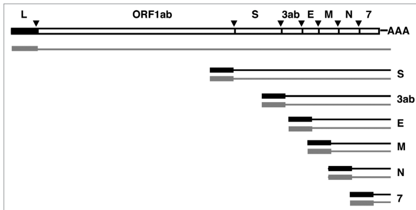
Figure 1. CoV genome structure and strategy of sgRNA expression. The upper line represents the TGEV genome structure. Letters above the bar indicate the gene names. L, leader sequence. AAA, poly(A). The shorter lines represent the viral mRNAs. Letters to the right of these lines indicate the gene encoded by each mRNA. Black lines represent the positive stranded RNAs, whereas gray lines represent the negative stranded RNAs. The triangles indicate the positions of the conserved core sequences (CSs) located upstream of each gene.
