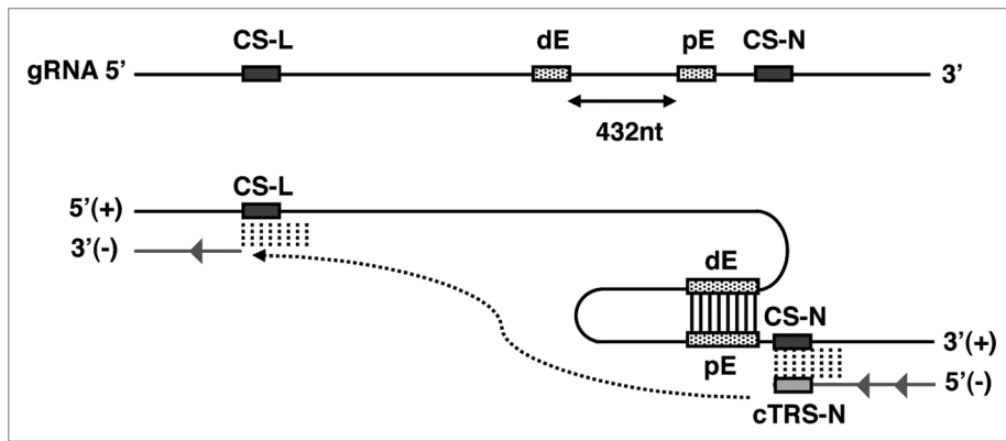
Figure 5. Working model for the specific regulation of TGEV sgRNA-N transcription. The upper line represents the TGEV genome (not to scale) including the core sequence (CS-L) located at the 3' end of the leader, the distal and proximal elements (dE and pE, respectively) and the CS of N gene (CS-N). The number below the arrow represents the distance between dE and pE elements. The lower lines represent the long distance RNA-RNA interaction within the genome that may act as a stop signal during the synthesis of the negative stranded sgRNA-N (gray line). The dashed arrow indicates the template switch step. cTRS-N, sequence complementary to the CS-N and the 3' TRS-N flanking sequences.
