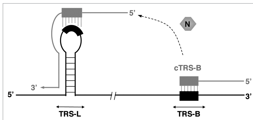
Figure 4. Postulated template switch during CoV transcription. Nascent minus RNA strand (gray) is synthesized by the RdRp using genomic RNA (black) as a template. After template switch (indicated by the dashed arrow), nascent minus RNA strand hybridizes with the TRS-L, to resume synthesis of the subgenomic RNA. Different viral and cellular proteins may be involved in this process. N protein is required for an efficient transcription, and may help template switch by acting as an RNA chaperone.
