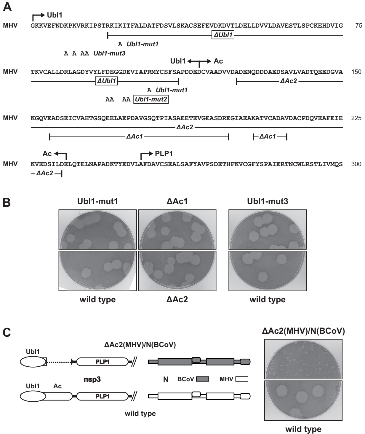
FIG 6 MHV Ubl1 and Ac mutants. (A) Sequence of the amino-terminal region of MHV nsp3. Constructed Ubl1 and Ac point mutations and deletions are indicated; lethal mutations are boxed. (B) Plaques of viable Ubl1 and Ac mutants at 37°C compared with those of the wild type. (C) Failure of the ΔAc2 mutation to complement the BCoV N substitution. Plaques of the ΔAc2(MHV)/N(BCoV) mutant at 37°C are compared with those of the wild type. Plaque titrations for panels B and C were carried out on L2 cells; monolayers were stained with neutral red at 72 h postinfection and were photographed 18 h later.
