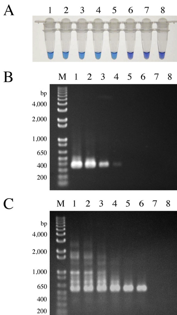
Fig. 2. Visual inspection of sensitivities of NATs, A, RT-LAMP after 90 min incubation; B, RT-PCR; and C, nested RT-PCR. Lane M, 1 kb Plus DNA ladder (Life Technologies Japan); tubes (lanes) 1–7, 10-fold serially diluted MHV-3 RNA from 10^3 to 10^9 ; tube (lane) 8, negative control.
