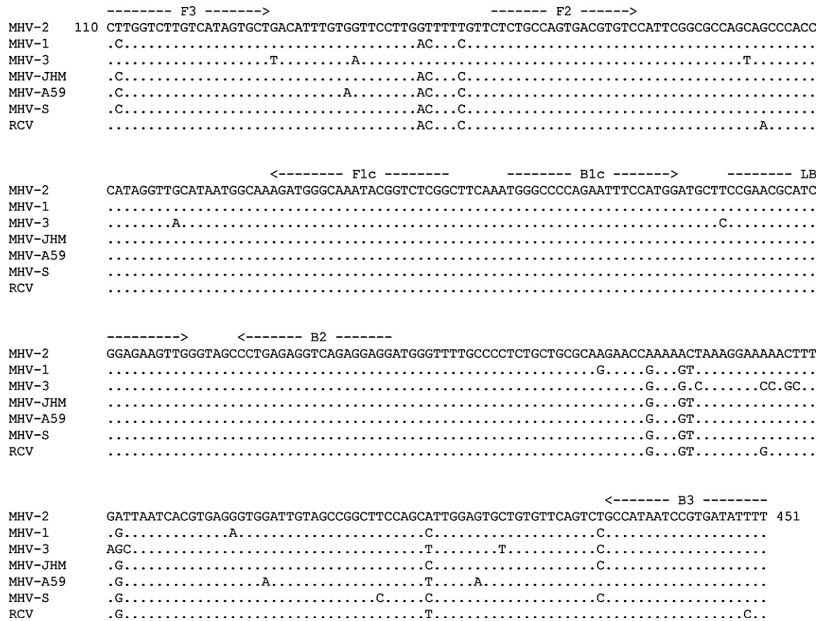
Fig. 1. Sequence alignment of rodent coronavirus genes between the F3 and B3 primers. Numbers at the beginning and end of sequences denote the nucleotide positions of MHV-2 (GenBank ID: AF201929). Arrows indicate the sequences from the 5' to 3' end used for the respective primers, and nucleotides that matched those of MHV-2 are represented as dots. FIP and BIP primers contain two distinct sequences: F1c plus F2 and B1c plus B2, respectively.
