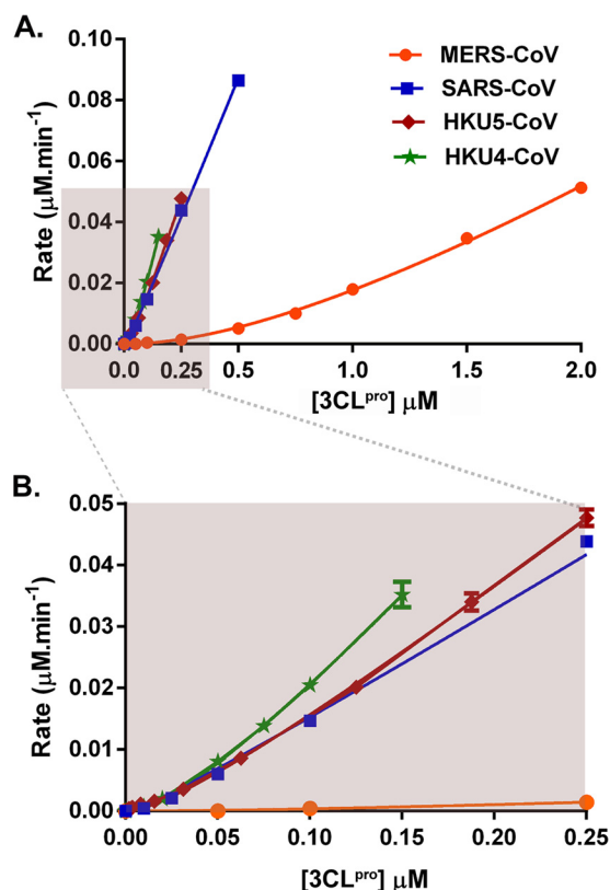
FIGURE 2. Dependence of the enzymatic activity of MERS-CoV, HKU4-CoV, HKU5-CoV, and SARS-CoV 3CL pro on the total enzyme concentration. A, kinetic response of each CoV 3CL pro to increasing enzyme concentration is plotted along with the resulting fit of the data to Equation 2. Resulting values for the apparent turnover number, k_{cat} , and the monomer-dimer equilibrium constant, K_d , are shown in Table 2. Final enzyme concentrations varied over the concentration ranges of 2 \mu\text{M} to 100 nM for MERS-CoV 3CL pro , 500 to 10 nM for SARS-CoV 3CL pro , 250 to 0.6 nM for HKU5-CoV 3CL pro , and 200 to 10 nM for HKU4-CoV 3CL pro . Final substrate concentration was fixed at 2 \mu\text{M} . Experiments were done in triplicate. Error bars represent the standard deviation for triplicate data. Shaded box represents the data that are plotted in B. B, enlarged view of the fitted data at low total enzyme concentrations, marked in shaded box in A, illustrating the nonlinear dependence of enzymatic activity on the total concentrations of 3CL pro from SARS-CoV, HKU5-CoV, and HKU4-CoV.
