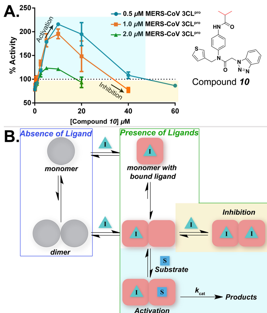
FIGURE 5. Activation of MERS-CoV 3CL pro via ligand-induced dimerization. A, enzymatic activity of 0.5, 1.0, and 2.0 \mu\text{M} MERS-CoV 3CL pro was measured in the absence and presence of varying concentrations of compound 10 . Substrate concentration was fixed at 2.0 \mu\text{M} . % activity, normalized to zero inhibitor enzymatic activity, was plotted as a function of increasing inhibitor concentrations. Error bars represent the standard deviation for triplicate data. Increase in enzymatic activity (highlighted in cyan-shaded box) is observed in the presence of low concentrations of compound 10 . Inhibition of enzymatic activity is observed at higher inhibitor concentrations (highlighted in yellow-shaded box). B, kinetic model describing the equilibrium between different species of MERS-CoV 3CL pro that are formed in the absence (blue box) and presence (green box) of a ligand is shown. Based on the AUC-calculated K_d value of \sim 52 \mu\text{M} , MERS-CoV 3CL pro primarily exists as a monomer in solution in the absence of a ligand. Upon ligand binding (inhibitor I in our case) to the monomer, the monomer-dimer equilibrium shifts toward dimer formation. Next, under lower inhibitor concentrations (cyan-shaded box), substrate ( S ) binds in the second active site and catalysis takes place. However, under higher inhibitor concentrations (yellow-shaded box), inhibitor directly competes with the substrate for the second active site, and inhibition of the enzymatic activity is observed.
