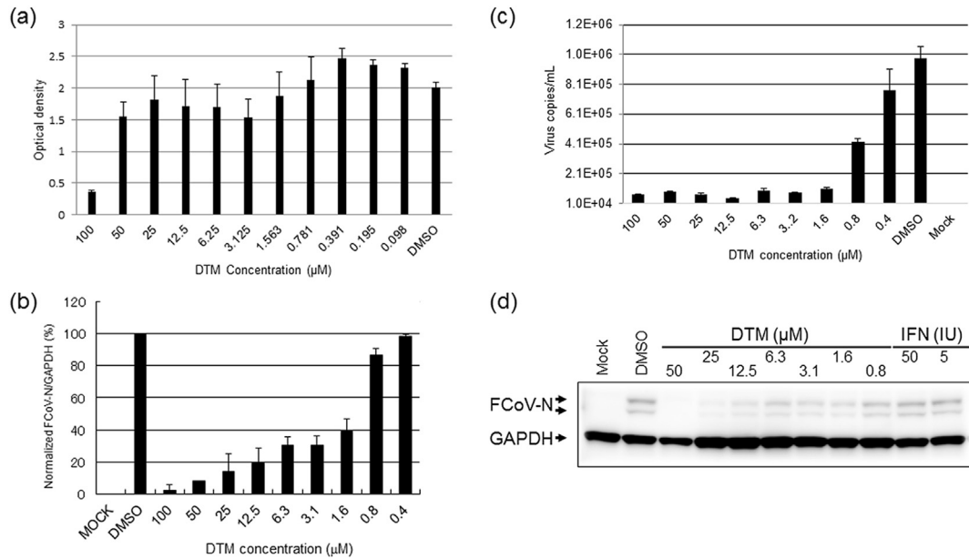
Fig. 3. DTM, a specific Pin1 inhibitor, inhibits FCoV replication. (a) fcwf-4 cells were incubated with DTM to examine cell toxicity using various concentrations of DTM. After 24-h treatment with DTM, cell viability was assessed by the WST-8 assay. Error bars indicate standard deviations. (b) fcwf-4 cells treated with various concentrations of DTM were infected with FCoV. At 20 h after infection, the cells were collected with cell lysis buffer and analyzed by Western blotting methods. DMSO not containing DTM was used as a positive control lane. (c) Total RNAs from the supernatants of infected cells were treated as described in the panel legend (b) and were extracted and analyzed by RT-qPCR. Each sample was assessed through triplicate measurements. Error bars indicate standard deviations. (d) fcwf-4 cells were incubated with or without DTM and IFN- \omega after infection with FCoV. At 20 h after infection, the cells were lysed with cell lysis buffer and assessed by Western blotting analysis.
