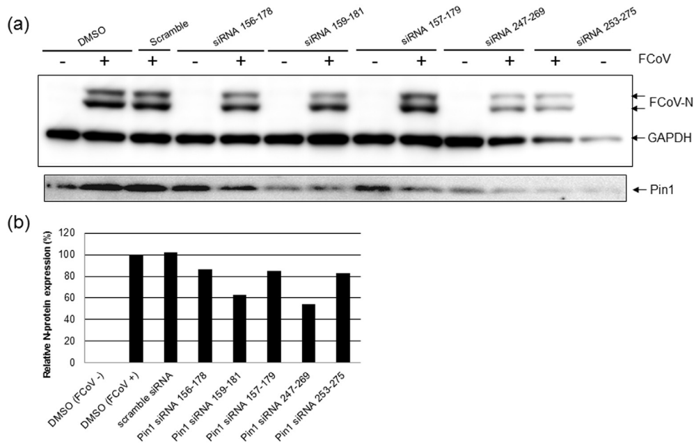
Fig. 4. fcwf-4 cells were transfected with various kinds of siRNA against Pin1 gene. (a) At 24 h after transfection, the cells were infected with FCoV and incubated for 20 h. Total cell lysates after incubation were assessed by Western blotting. Scramble siRNA was used for a negative control experiment. (b) Relative FCoV-N protein expression was normalized with GAPDH protein from the results of panel (a), and Western blotting experiments were indicated.
