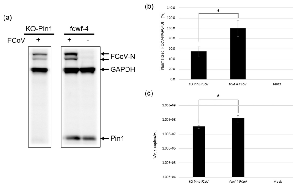
Fig. 5. KO cells for the Pin1 inhibit FCoV replication. (a) Stable KO cells for the Pin1 gene were infected with FCoV. At 20 h after infection, total cell lysates were prepared and used for Western blotting analysis. (b) Relative FCoV-N protein expression was normalized with GAPDH protein from the results of panel (a), Western blotting experiments were indicated. Each sample was assessed by triplicate measurements. Error bars indicate standard deviations. The asterisk indicates a significant difference (*, p < 0.05 ) from the value for the parent fcwf-4 cells. (c) Total RNAs from the supernatants of infected cells treated as described in the legend to panel (a) were extracted and analyzed by RT-qPCR. Each sample was assessed by triplicate measurements. Error bars indicate standard deviations. The asterisk indicates a significant difference (*, p < 0.05 ) from the value for the parent fcwf-4 cells.
