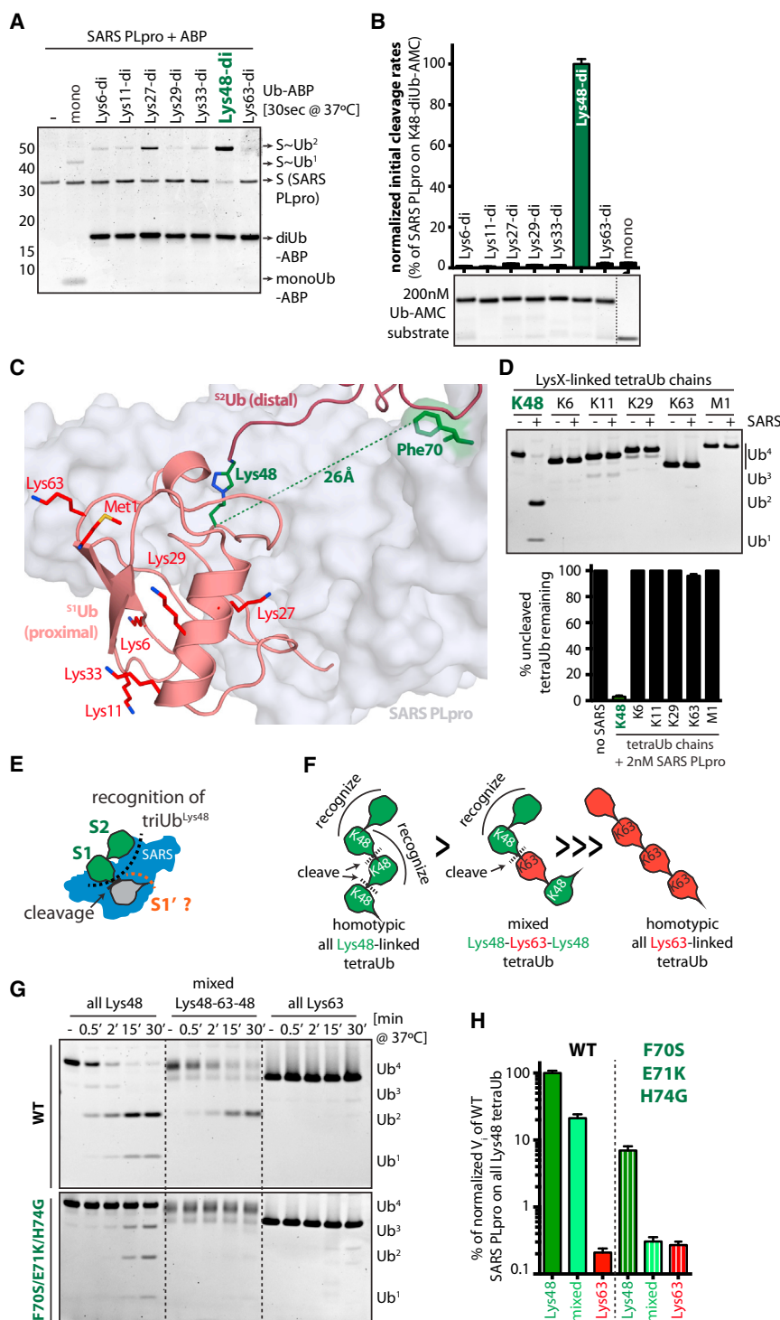
Figure 4. SARS PLpro Activity Is Restricted to Lys48-Linked Ub Chains with Specificity Dominated by S2-S1 Interactions
