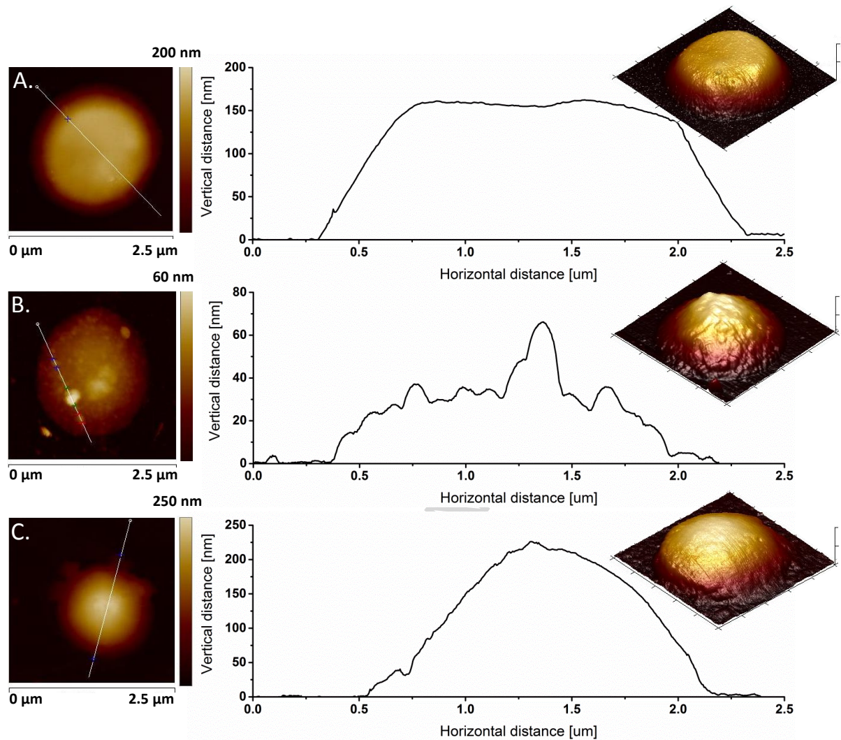
Figure 3. H-HTCC NS/MS bind HCoV NL63 virions. Height, cross section and 3D AFM topography images of H-HTCC-MS incubated with lysate of mock infected (A) or virus infected (B) cells. H-HTCC-NS/MS imaged after desorption with 2 M NaCl (C). Scan size: 2.5 x 2.5 \mu\text{m} for 2D figures. Scan size and the vertical scale on 3D figures: 2.5 x 2.5 \mu\text{m} and 100 nm (A); 2.0 x 2.0 \mu\text{m} and 50 nm (B); and 1.0 x 1.0 \mu\text{m} and 100 nm (C), respectively.
