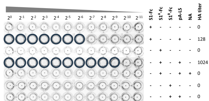
Fig. 4. MERS-CoV S1-mediated Sia-binding activity resides in S1 A . MERS-CoV S1-, S1 A -, and S1 B -Fc proteins alone or complexed with pA-LS were subjected to hemagglutination assay using human erythrocytes, after which HA titers were determined. MERS-CoV S1 A -Fc hemagglutination activity was additionally tested with NA-treated human erythrocytes. Wells positive for hemagglutination are encircled. Hemagglutination assays were performed at least two times.
